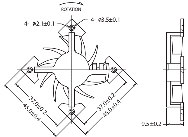
DIMENSIONS DRAWING
