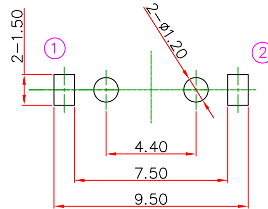
RECOMMENED P.C.B MOUNTING PATTERN DIMENSION
