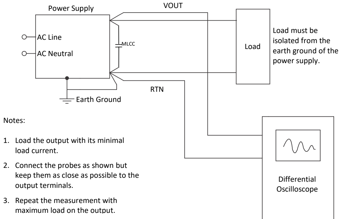
Figure 3-3 Ripple Noise Measurement Setup
