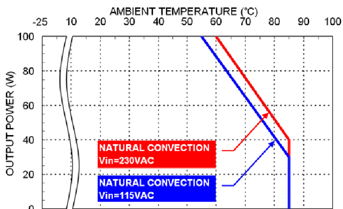
Derating Curve vs. Ambient Temperature XLE100 and XLD100
