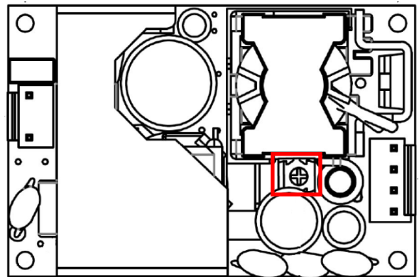
Figure 3-4 Potentiometer for V1 Output Adjustment
