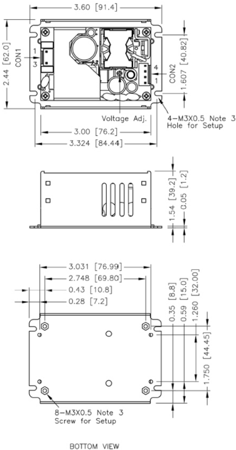
Figure 4-3 Mechanical Drawings (All Models)
