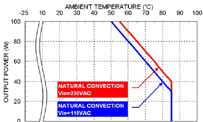
Derating Curve vs. Ambient Temperature XLO100 and XLU100
