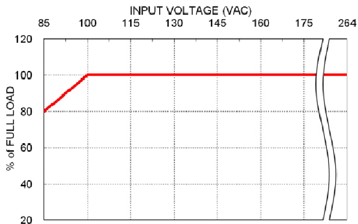
Figure 3-2 Load vs. Input Voltage
