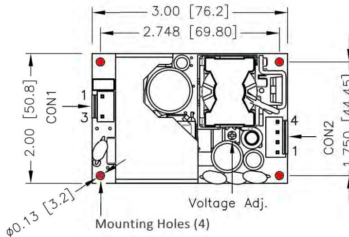
Figure 4-2 XL100 Mounting Hole Locations
