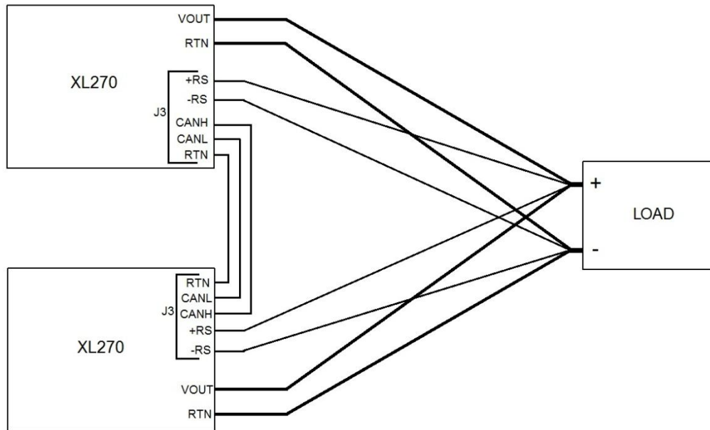
Figure 3-5 Current Share Wiring Example – Two XL270's.
