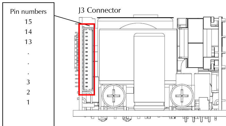
Figure 4-3 J3 Connector
